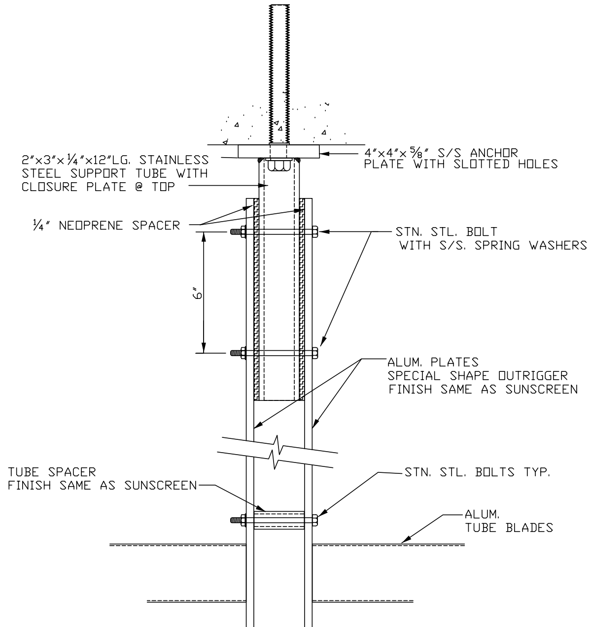
SECTION DETAIL
